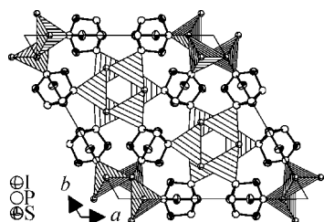
Figure 2. Section of the crystal structure of (CuI)_3P_4S_4 . \beta - P_4S_4 cages are coordinated through P1, P2, and P2' to copper atoms within the tetrahedra. Notice the different orientation of the tetrahedra within different columns.
